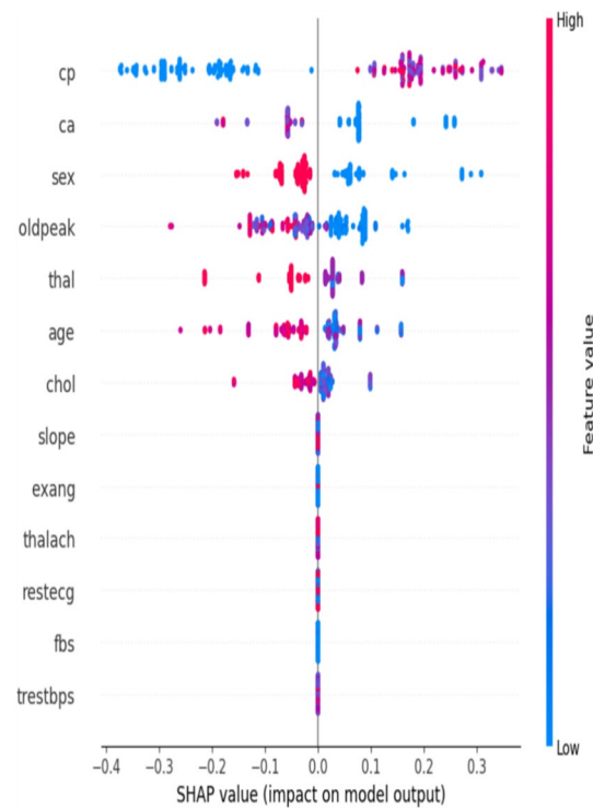
Fig. 8 Summary plot of the proposed ensemble approach
