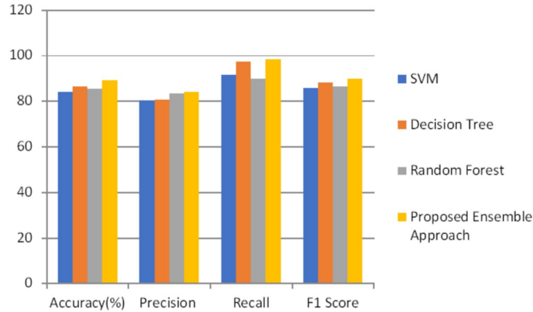
Fig. 3 Comparison of performance evaluation of proposed and baseline ML models
