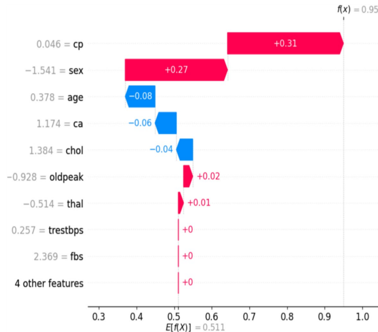
Fig. 5 Waterfall plot of the proposed ensemble approach
